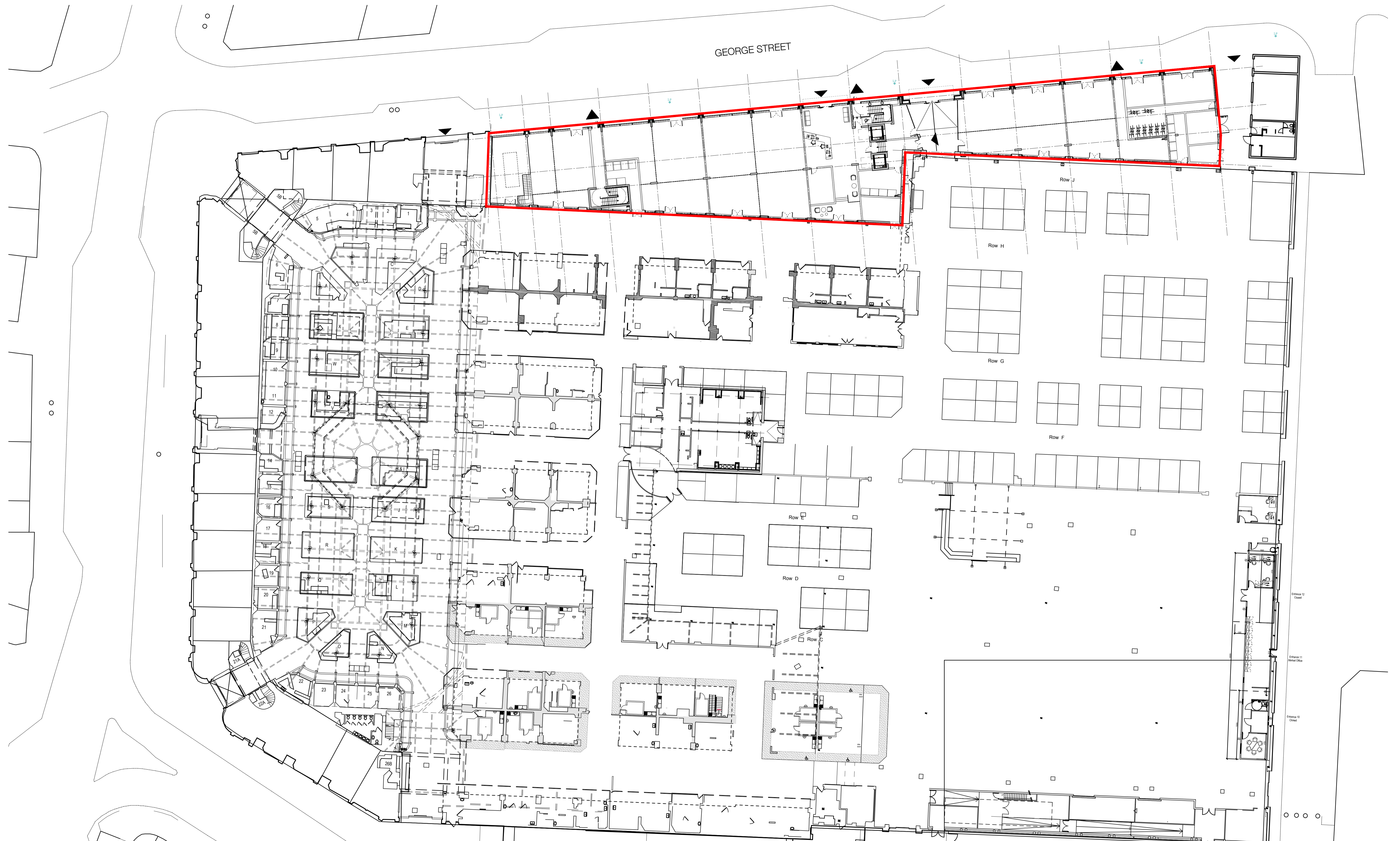
(10)1000 Ground Floor Plan Scale - 1:150 @ A1
