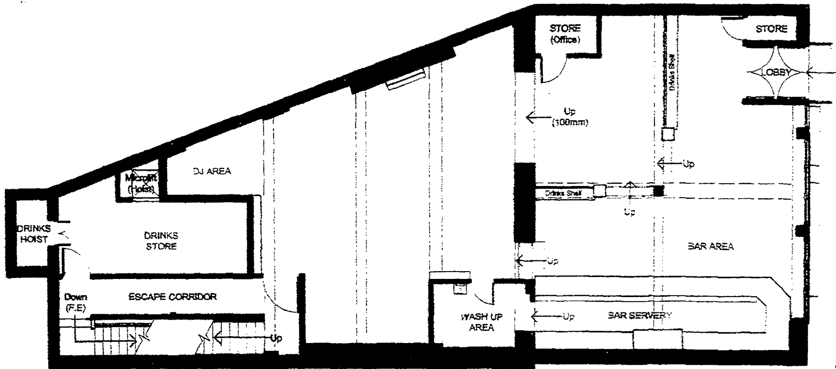
SUBURBAN STYLE BAR - EXISTING GROUND FLOOR PLAN @ 1:100
