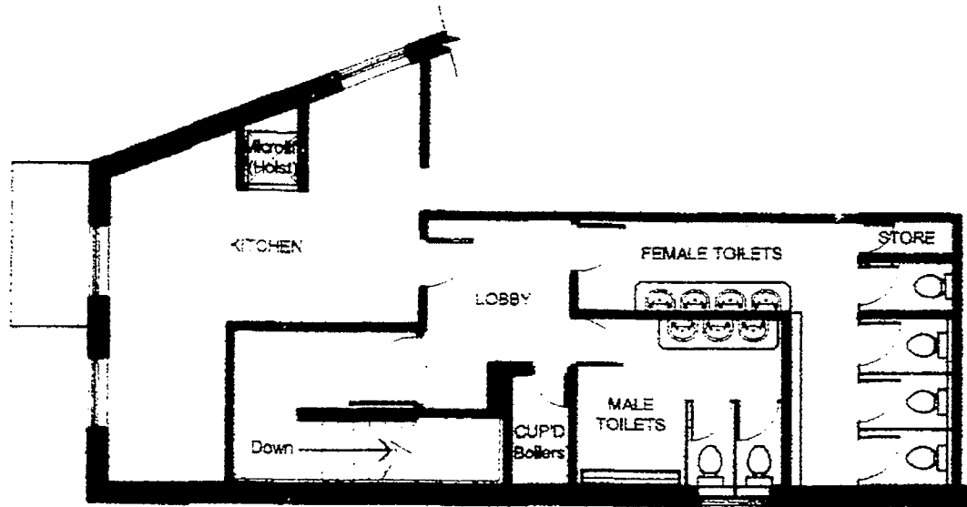
SUBURBAN STYLE BAR - EXISTING 1st FLOOR PLAN @ 1:100
